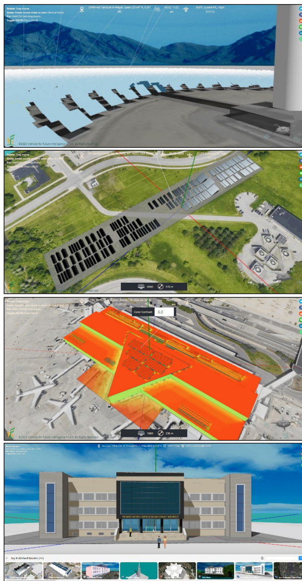
FIGURE 5. Aladdin as a citizen science platform for modeling and/or designing real-world projects. From top to bottom: The PS20 solar power tower in Seville, Spain; The Solar Strand at the University of Buffalo, New York, USA; Solar panel arrays on the roof of Terminal A, Logan International Airport, Boston, USA; The BILSEM science education center in Mersin, Türkiye.
